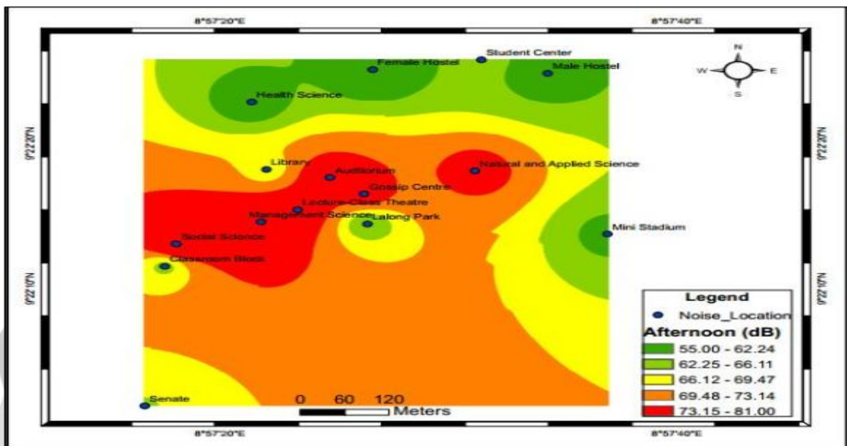
Figure 3: Noise Level in the Afternoon at Plateau State University, Bokoos
