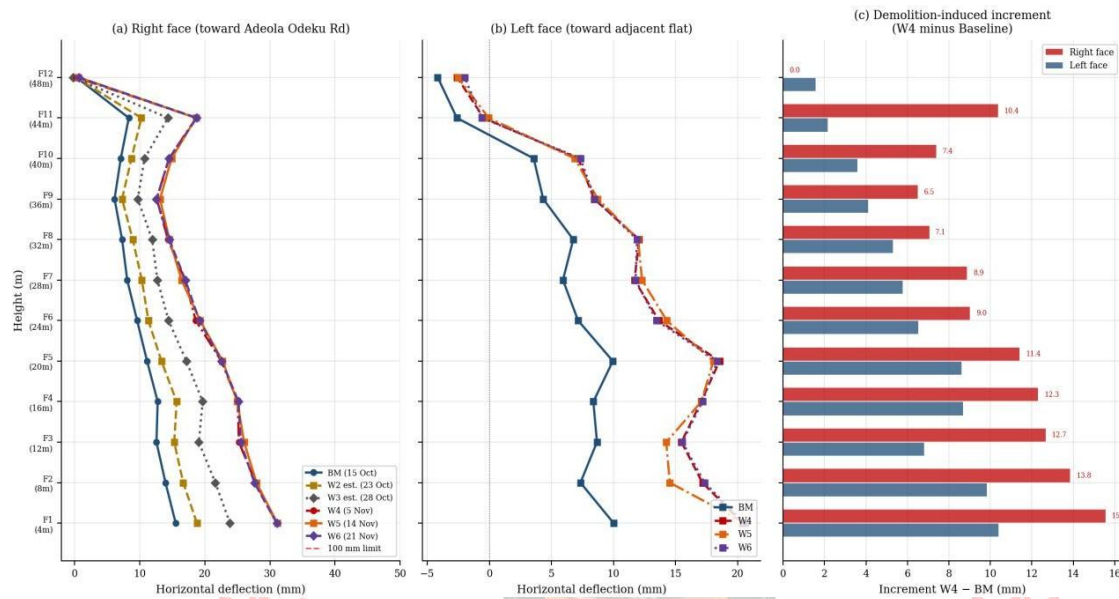
Figure 2. Total Station deflection profiles by floor level. (a) Right-face profiles all campaigns; (b) Left-face profiles; (c) Incremental deflection W4 minus baseline (d) Multi-campaign bar chart; (e) Height–deflection polynomial regression (F1–F11); (f) Deflection growth rate BM→W4.
